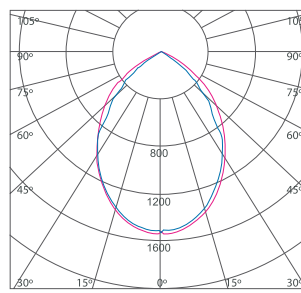
cd/klm C0/C180: C90/C270: HS-HL-50W
