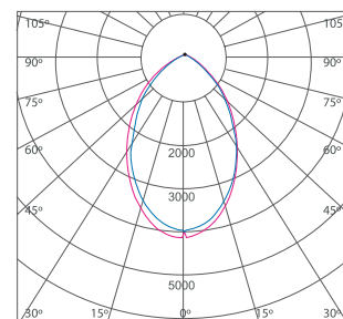
cd/klm C0/C180: C90/C270: HS-HL-100W
